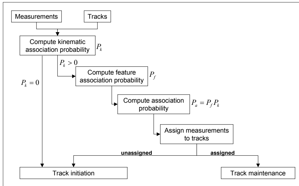
Figure 1: Signature-Aided Association
